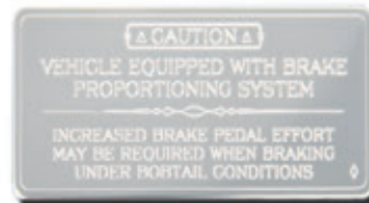
KT-952BP S/S - Statement Plate - Brake Proportioning
